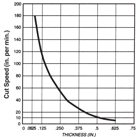
HandyPlasma® 550 / PT-31XL Cutting Performance
