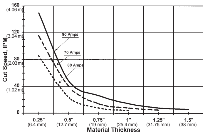
PT-32EH CUTTING SPEEDS OUTPUT CURRENT 60, 70 & 90AMPS w/AIR @ 75psi (5.2bar)
